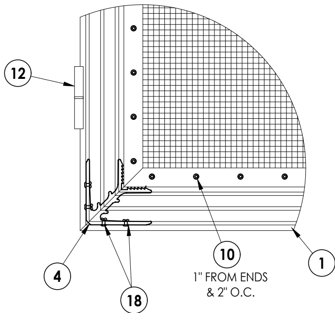
SCREEN DOOR CORNER DETAIL
