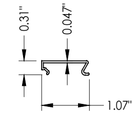
19 COVER
