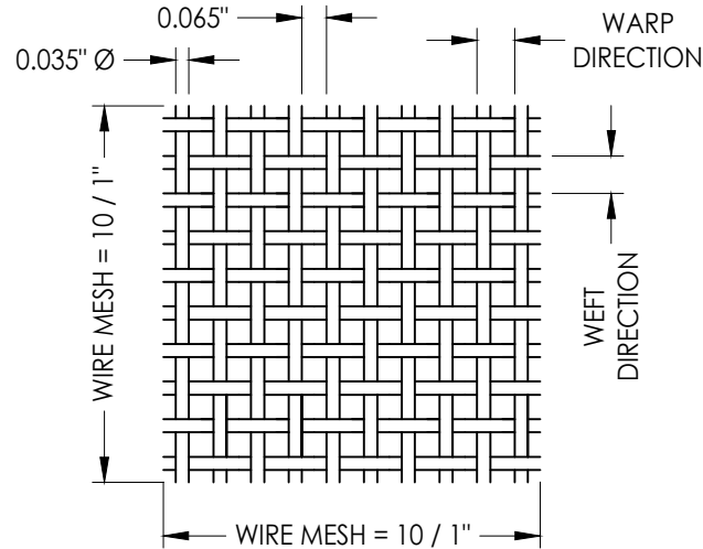
WIRE MESH (10 x 10) 304 Stainless Steel Wire Ø = 0.035" Open Area = 42.25%
