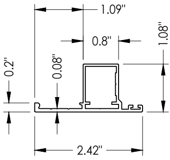
3B FACE MOUNT DOOR BUILD-OUT
