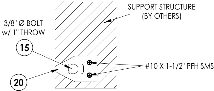
SLIDE BOLT STRIKE PLATE DETAIL (Shown @ Sill - Head Similar)
