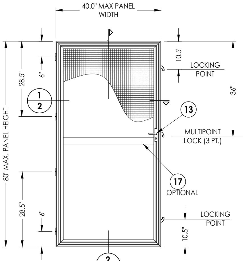
40 SCREEN DOOR PANEL
