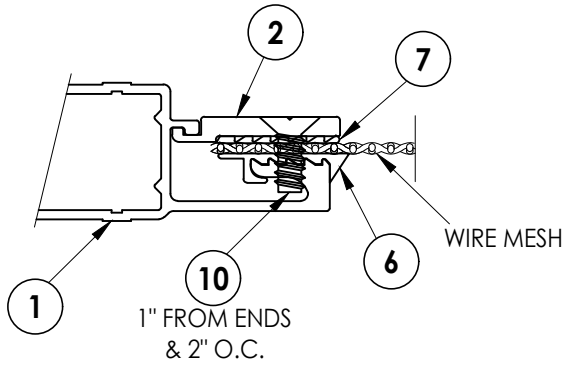
SCREEN CAPTURE DETAIL
