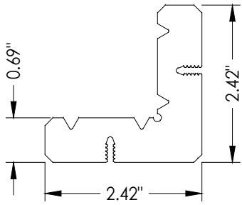
15 FRAME CORNER
