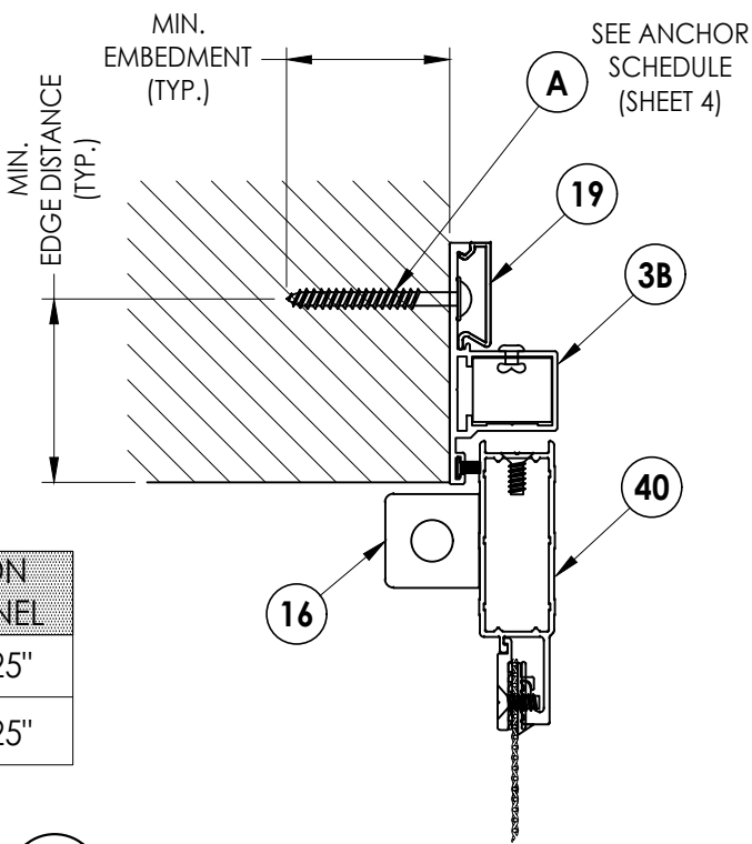
3 3 VERTICAL CROSS SECTION SHOWN w/ FACE MOUNT DOOR BUILD-OUT
